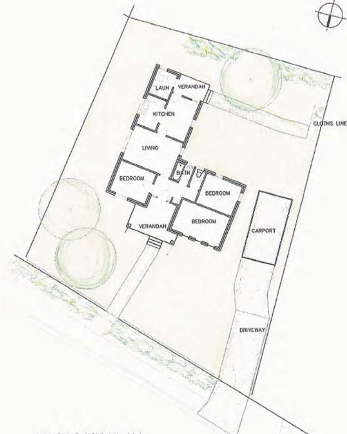
PROPOSED PLAN
