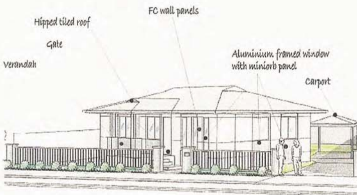
VIEW OPTION 2
