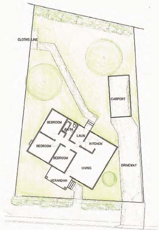
PROPOSED PLAN
