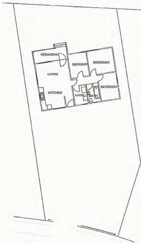
EXISTING PLAN
